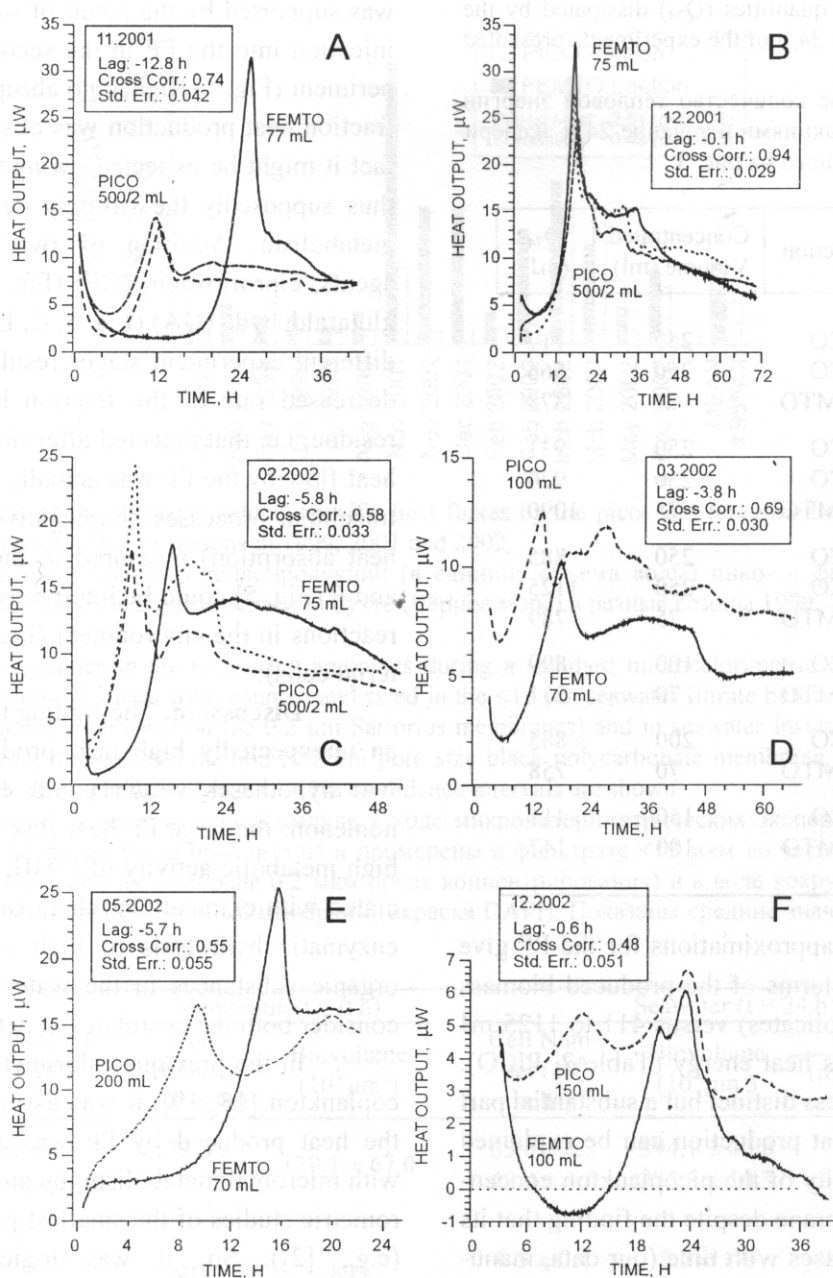
Fig. 3. The similarity between the heat flow patterns obtained for the plankton pico- and femtofractions from Sevastopol Bay (the Black Sea) in different seasons of 2001 and 2002. Each graph represents replicate experiments with the same seawater sample. Dates of the experiments, concentrated volumes (ml) and results of the cross correlation (CC) analysis, namely the maximum CC between the femto- and picofraction heat traces, its lag and standard error are shown. The volume of 500/2 ml means that after concentrating 500 ml of the fraction onto the membrane, the latter was cut into 2 equivalent fragments for conducting the replicate experiments.
