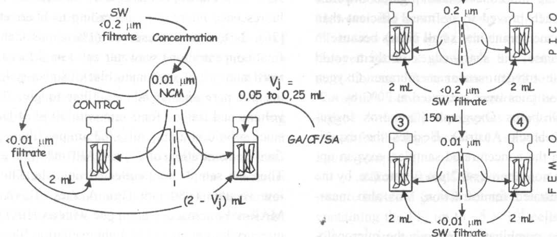
Fig. 1. Left : The 2-step filtration method for concentrating the femtofraction of seawater (SW) sample onto a nitrocellulose membrane (NCM). The membrane fragments of equivalent surface area were used to conduct replicate experiments with the unaltered samples and those subjected to glutaraldehyde (GA), ciprofloxacin (CF), and sodium azide (SA) treatments. V_j is the injection volume. Right : The experimental design used for monitoring the bacterial dynamics in measuring ampoules with the plankton PICO and FEMTO fractions. The numbers of the ampoules (in the circles), nominal pore sizes of the Sartorius nitrocellulose membranes, and the seawater (SW) volumes filtered and poured into the ampoules are shown. The experiment was conducted in 4 replicates.
