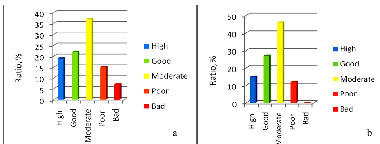
Fig. 4 Comparison of the ESC structure for water bodies of the Black Sea (a) (Northern Black Sea, 26 areas of Ukrainian part) and the Mediterranean Sea (b) (Western Mediterranean, 37 areas of Catalonia [4])
