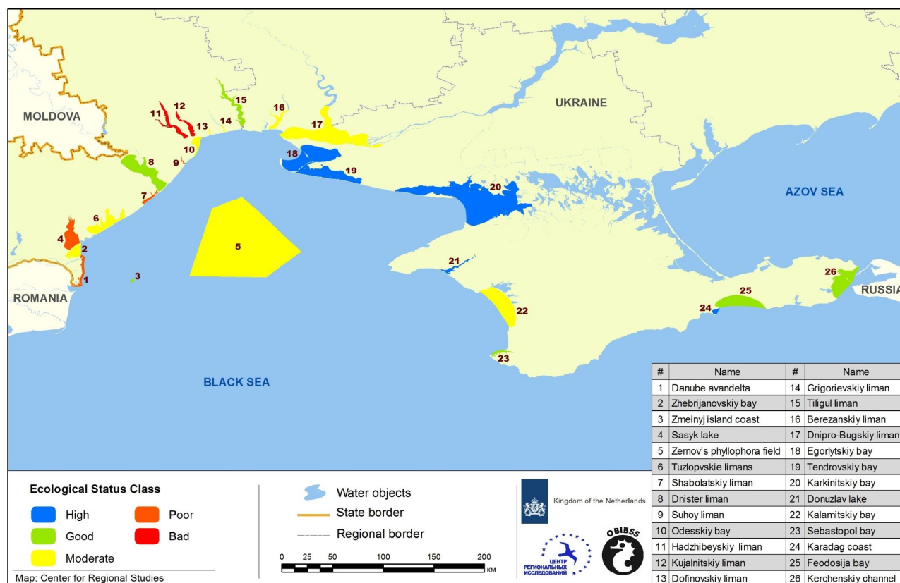
Fig. 3 Assessment of ESC of different water areas in the Ukrainian Northern Black Sea sector
