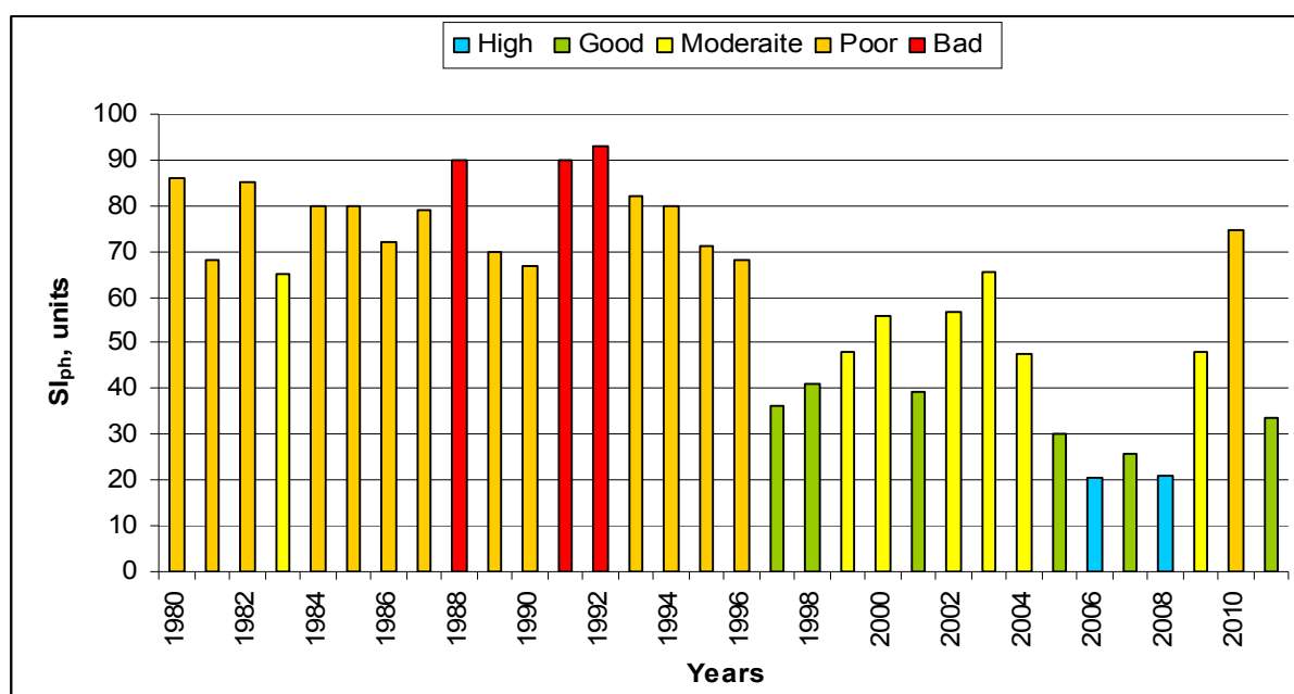
Fig. 5 Long-term dynamic of ESC value for Odessa coast (North-Western Black Sea) received using SI ph index
